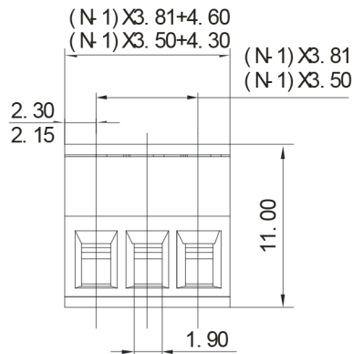
2EDGK-3.5 2EDGK-3.81
