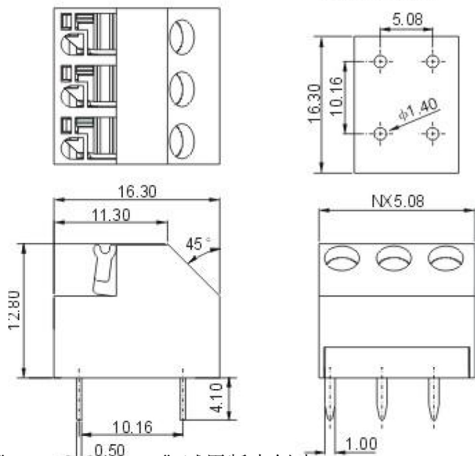
PCB LAYOUT
